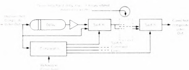
Simplified diagram of Delta 44 time base corrector.
